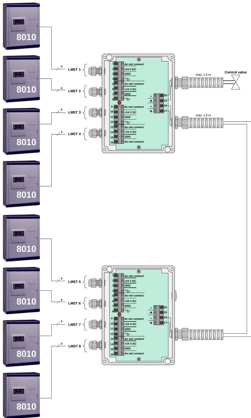
Fig. 40: Example for a Multisector-Control application
