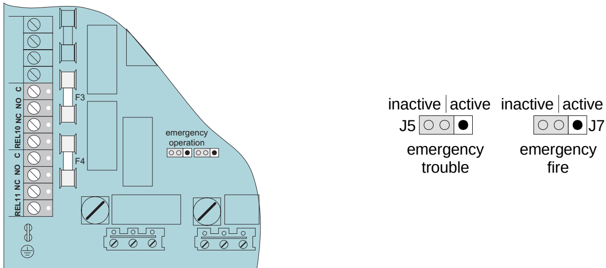
Fig. 33: Jumpers to configure the emergency operation function
