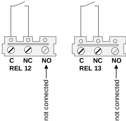
Fig. 29: Relays 12 and 13
