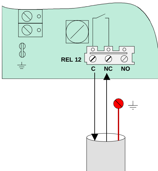
Fig. 30: Relay 12 (Example)
