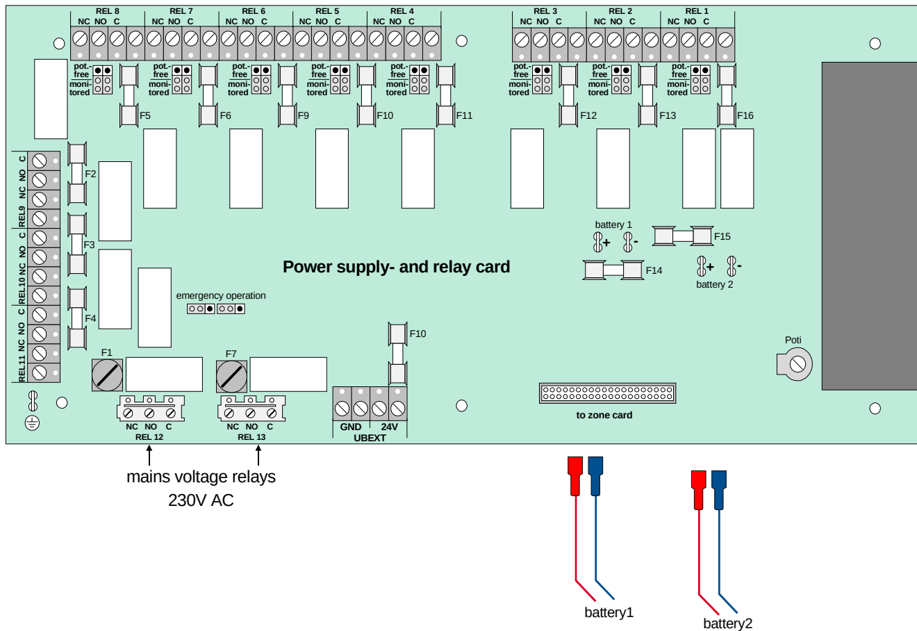
Fig. 28: Power supply unit and relay board / position of the subassemblies
