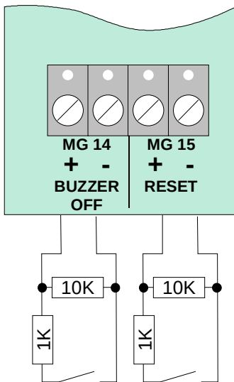
Fig. 27: Control input MG14 and MG15
