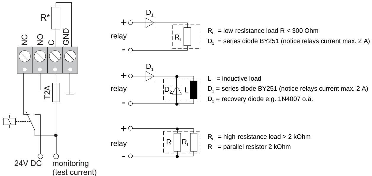
Fig. 32: Positive-switching / monitoring mode (Schematic wiring)
