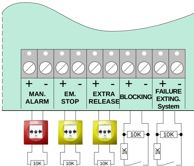
Fig. 26: Connecting the technical zones
