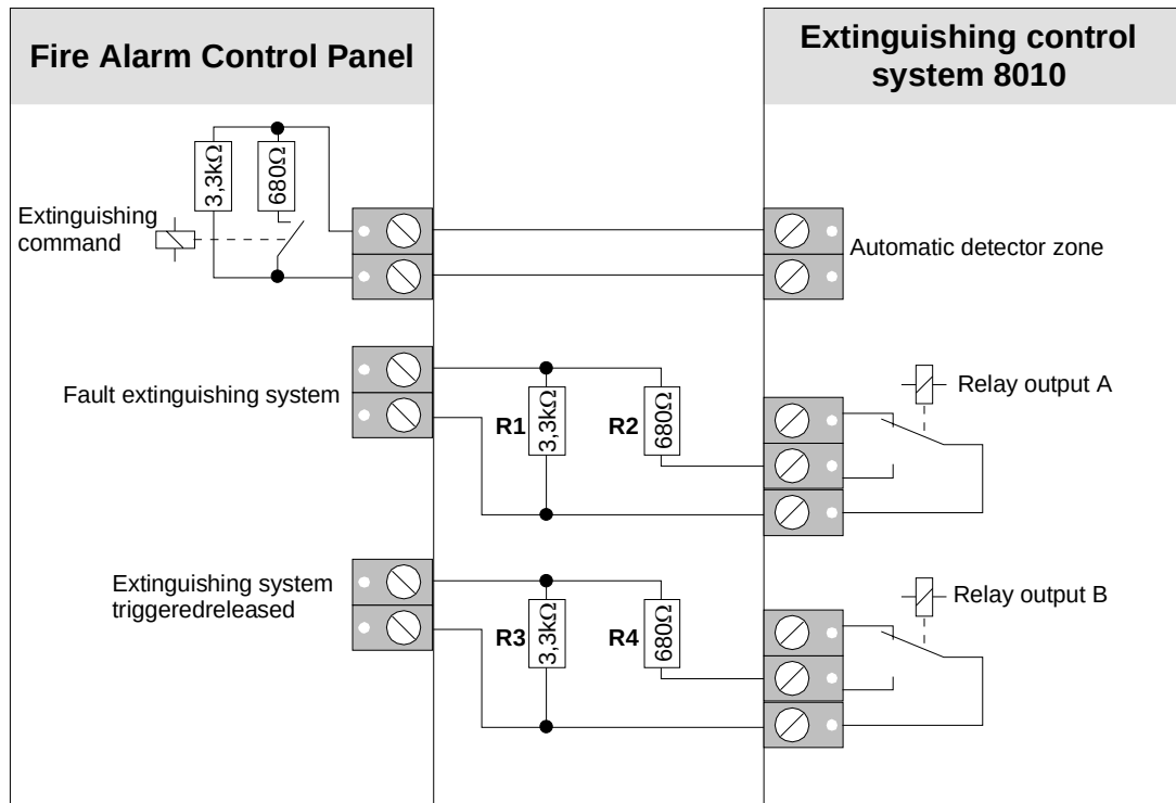
Fig. 34: Wiring of the interface
