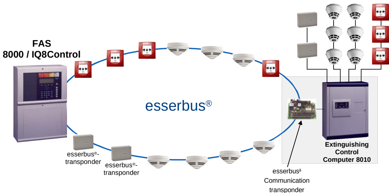
Fig. 39: Extinguishing Control Computer 8010 connected to the loop
