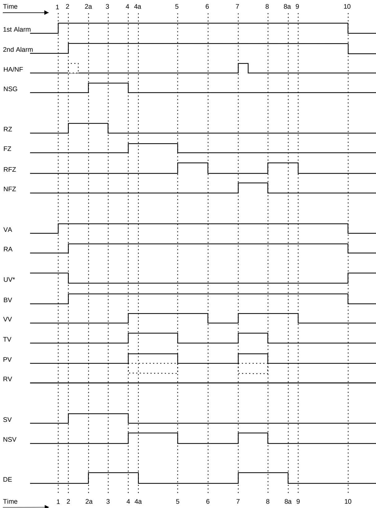
Fig. 36: Sequence diagram (Extinguishing System)
