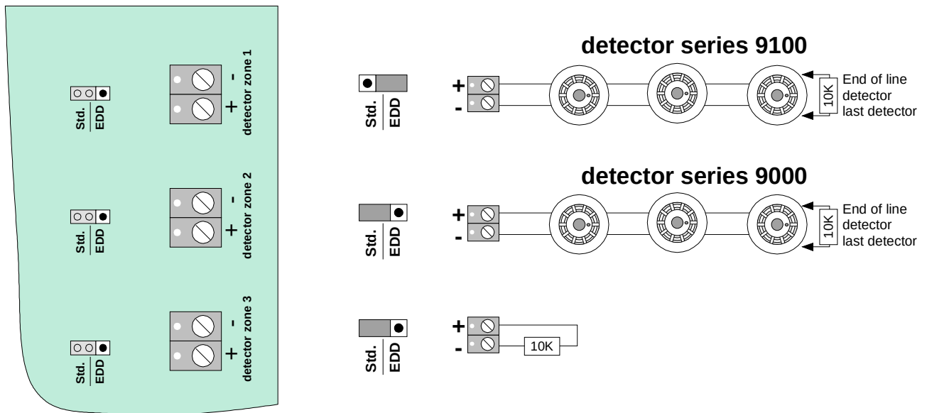
Fig. 25: Wiring of a fore alarm zone with detectors (schematic)
