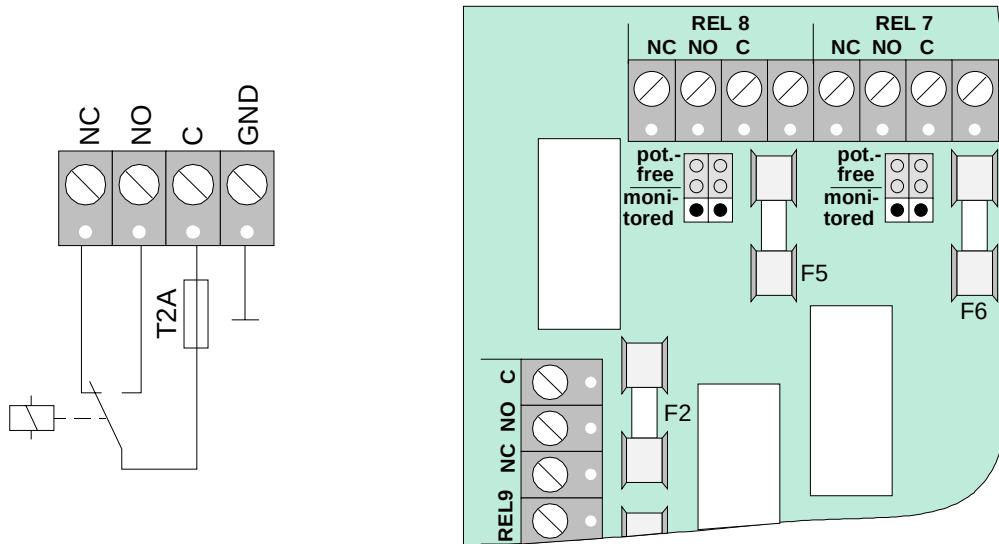
Fig. 31: Dry contact (Schematic wiring)
