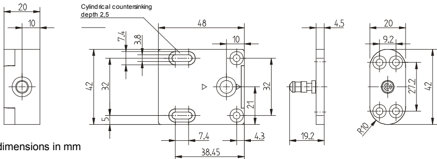
Illustration 3: Dimensioned drawing
